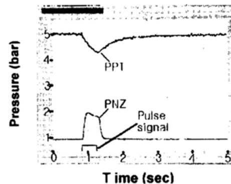
Fig. 9. The pressure traces in the pulse system during the pulse cleaning.
