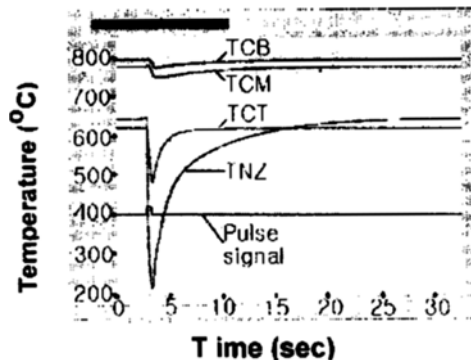
Fig. 7. The temperature traces during the pulse cleaning.
