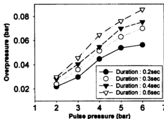
Fig. 12. The effect of the pulse pressure on the overpressure in the filter chamber.
