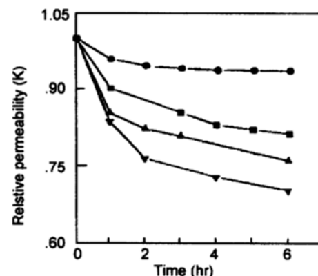
Fig. 3. The decrease of relative permeability with the pulse cycle duration; ● (5), ■ (10), ▲ (15) and ▼ (20 min).
