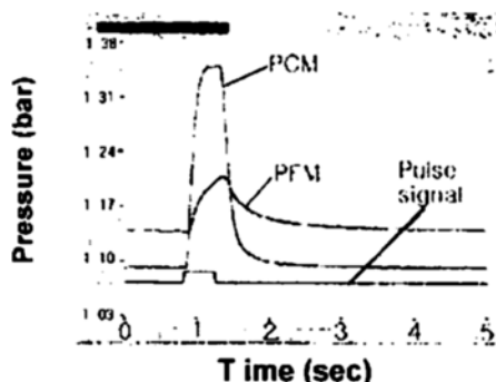
Fig. 10. The pressure traces in the filter cavity during the pulse cleaning.
